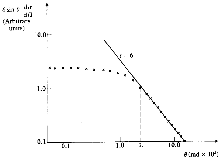
13.5 Log-log plot of \theta \sin \theta d\sigma/d\Omega vs \theta for the elastic scattering of potassium atoms by xenon atoms. The straight line corresponds to the classical cross-section for the potential V(r) = -A/r^s with s = 6 . The experimental data of Helbing and Pauly deviate from the classical result at very small angles ( \theta < \theta_c ) as expected (see text). For \theta < \theta_c agreement can be obtained with the data by calculating the cross-section using quantum methods. Notice from [13.38] that the shape of the classical cross-section is independent of the velocity of the atoms in the beams.
